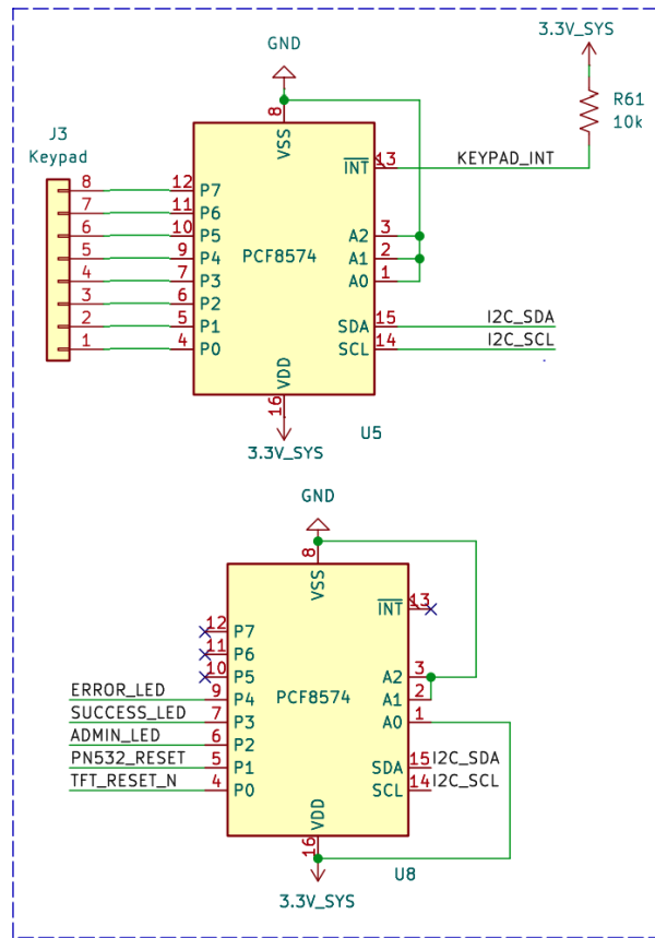
Figure 6.13 IO Bus Expanders Schematic
