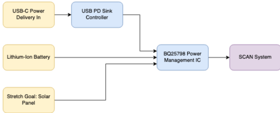
Figure 6.3 Power Delivery Block Diagram
