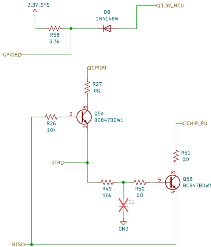
Figure 6.7 ESP32 Auto Downloader
