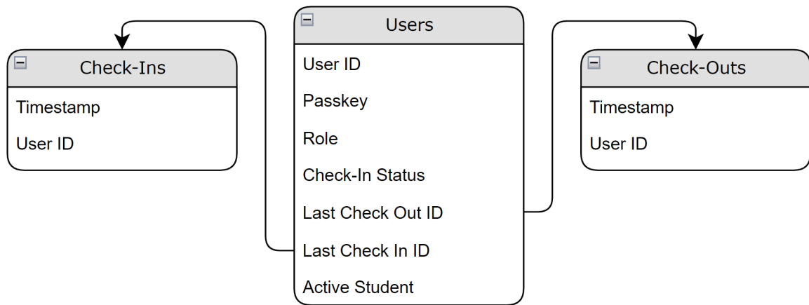
Figure 7.9 Database Fields
