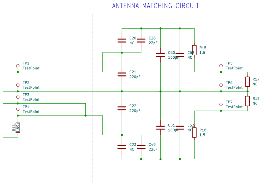
Figure 9.9 PN532 Antenna Probe Points
