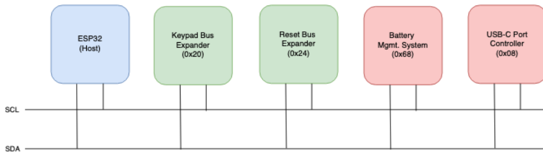
Figure 6.14 Shared I2C Bus Interface
