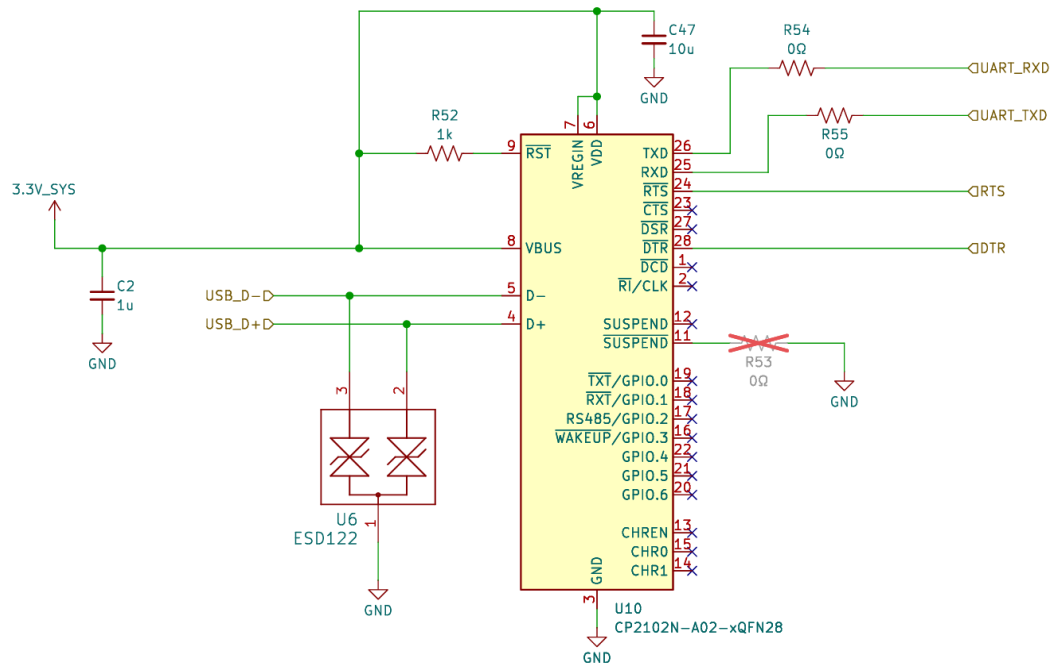
Figure 6.6 ESP32 USB-to-UART Bridge
