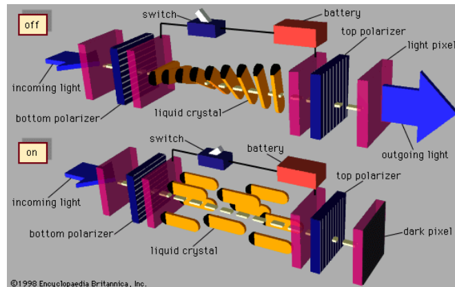
Figure 3.1 LCD Layer Composition (Obtained from Britannica)
