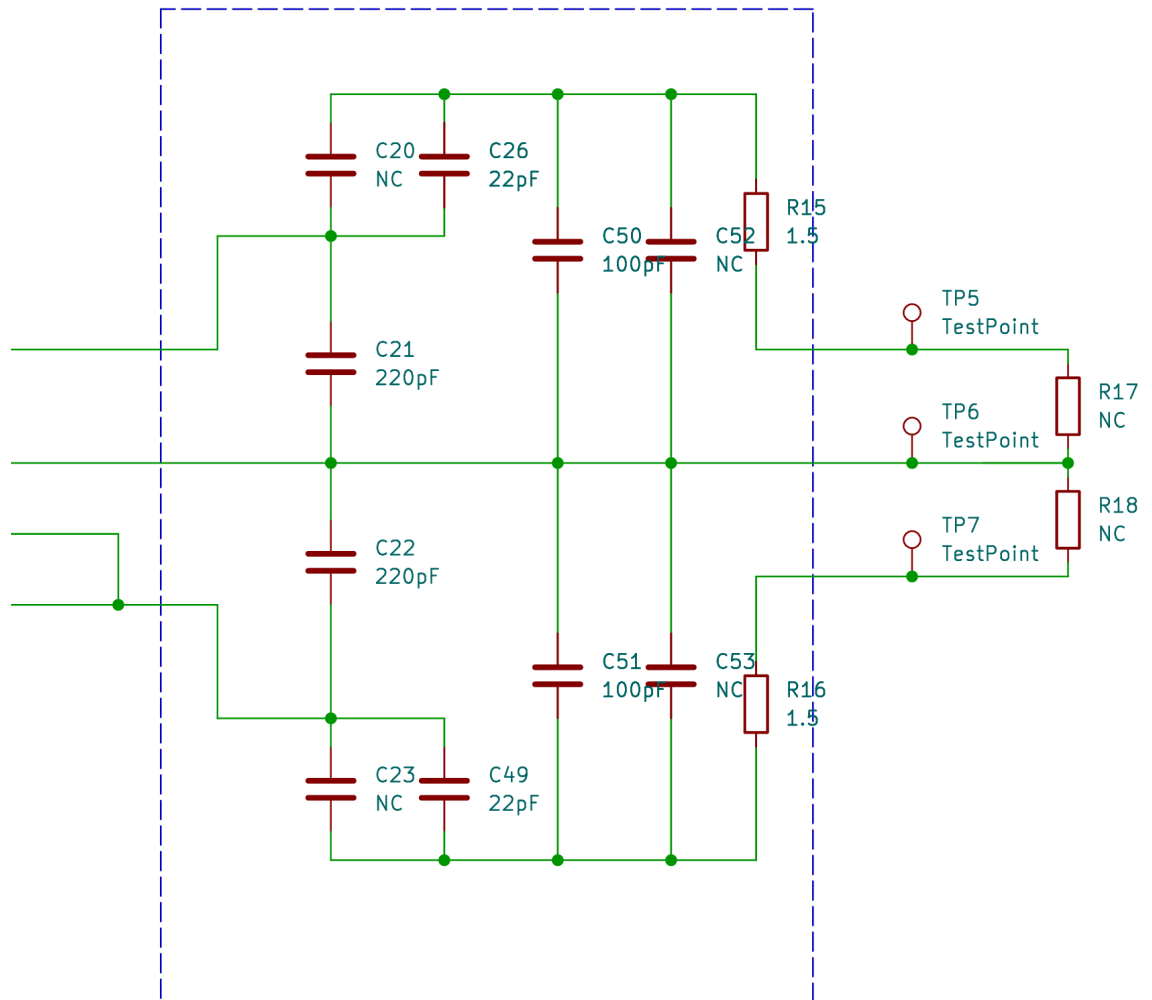
Figure 6.9 Antenna Matching Circuit
