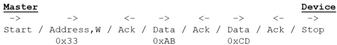
Figure 4.5 I2C Write Command (Obtained from embedded systems lab manual)
