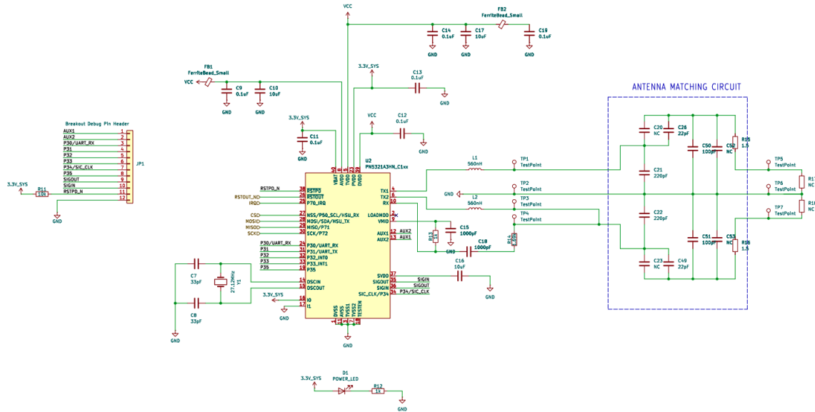
Figure 6.8 NFC Transceiver Schematic Design (Referenced from Adafruit)
