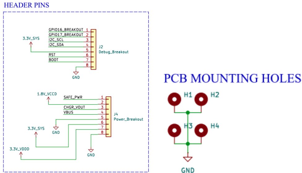
Figure 6.15 Breakout Pin Headers
