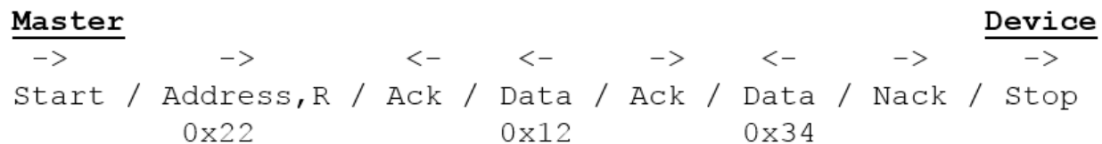
Figure 4.4 I2C Read Command (Obtained from embedded systems lab manual)
